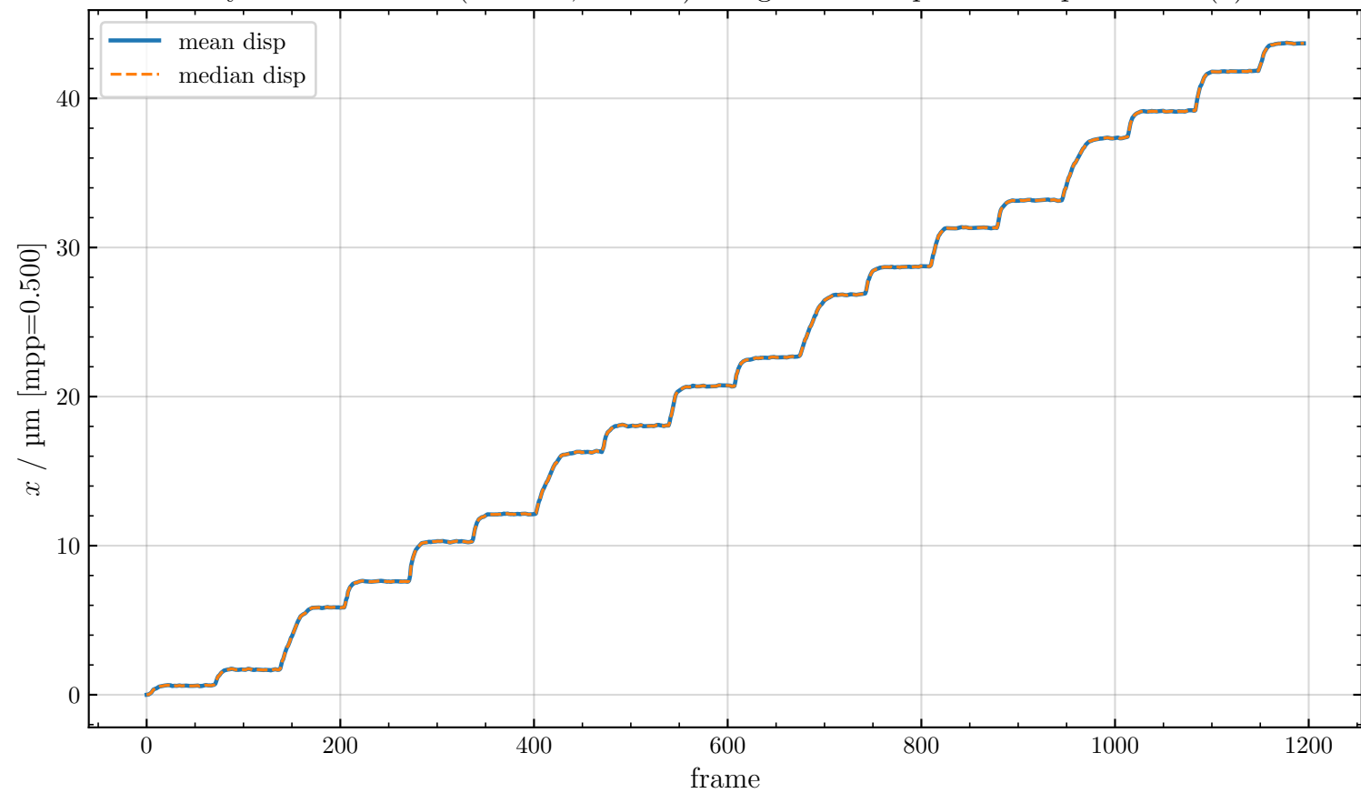
Dynabeads M-270 (2.00 Hz, 125 ms): Aligned mean particle displacement (1)
